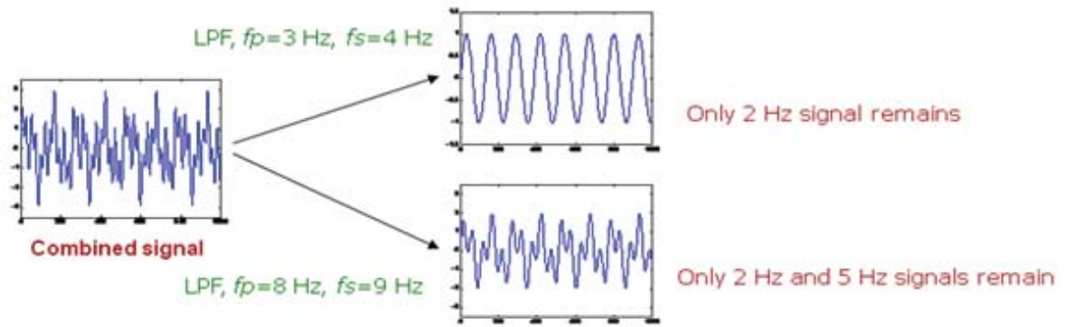
Figure 4.4: LPF of the three sinusoidal signals.
